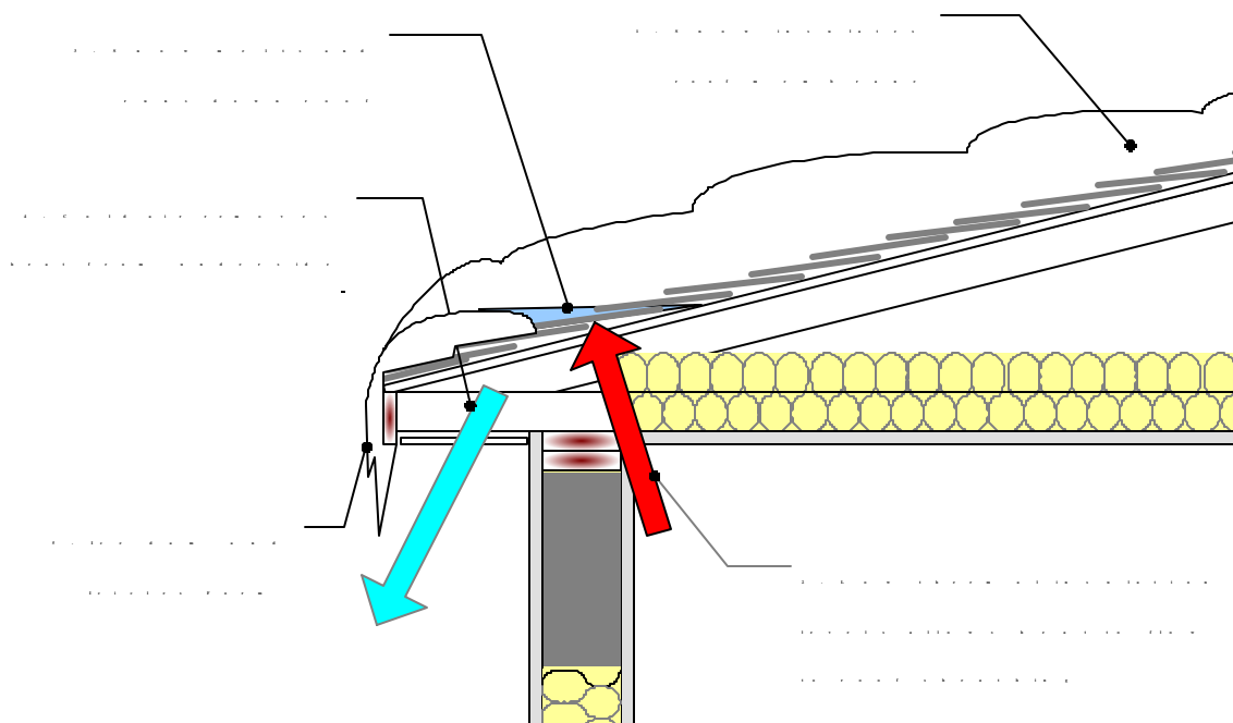
Figure 2: The Process of Ice Dam Formation Caused by Poor Insulation
