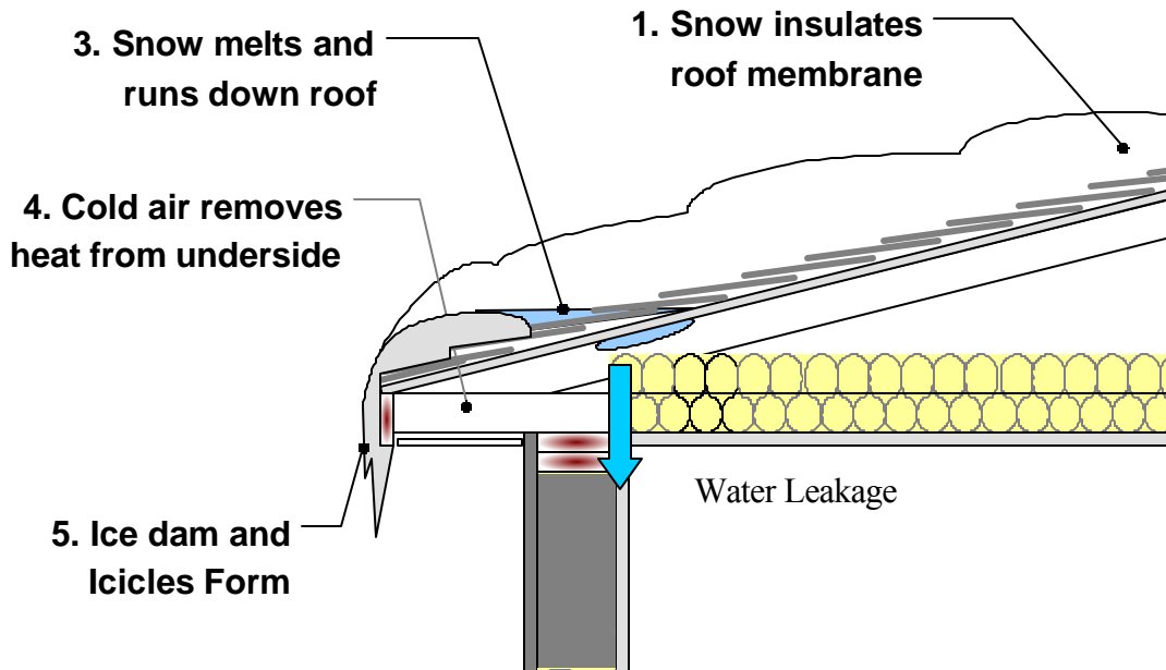
Figure 1: Ice Dam at a Typical Roof
