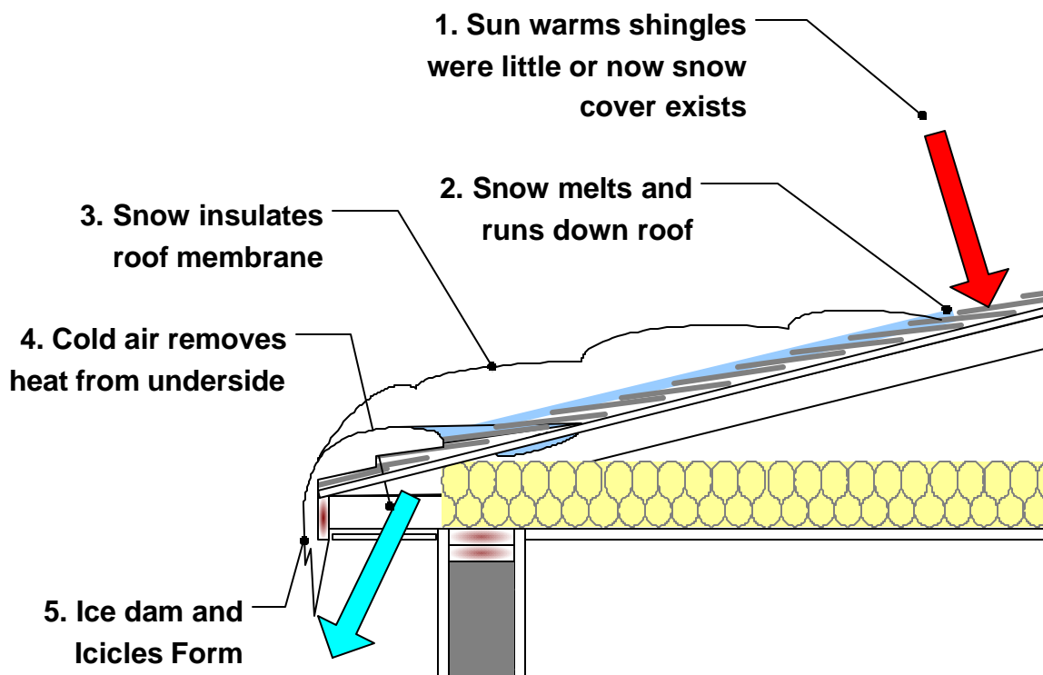
Figure 4: Ice Dam Formation Process Due to Uneven Snow Thickness
