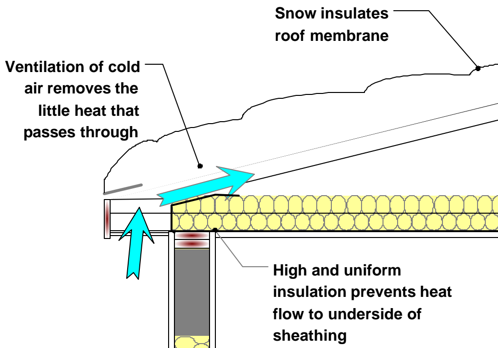
Figure 3: Solutions to Poor Insulation
