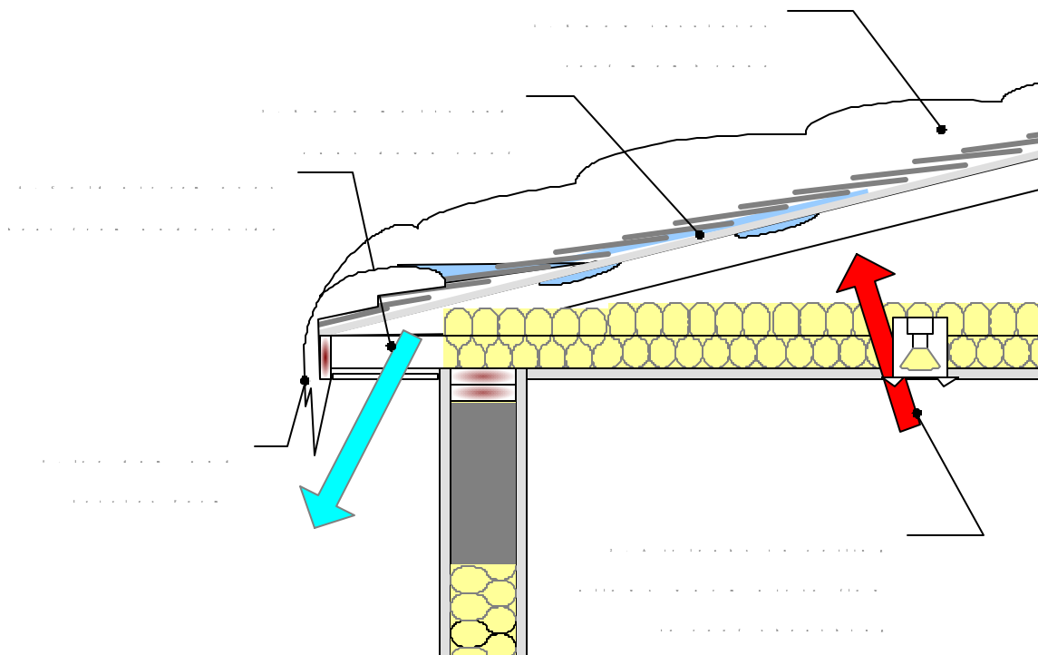
Figure 4: Ice Dam Formation Process Caused By Air Leakage
