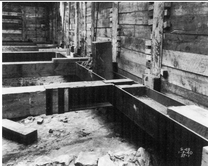
Braced cut in Chicago subway construction, January 1940 (courtesy of Ralph B. Peck)
