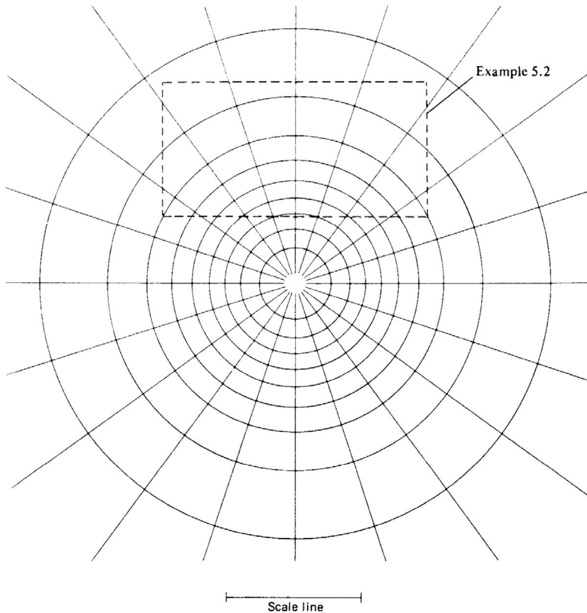
Fig. 5.11 Newmark's influence chart for vertical stress. Influence value per unit pressure = 0.005. (Reproduced from N.M. Newmark (1942) Influence Charts for Computation of Stresses in Elastic Foundations , University of Illinois Bulletin No. 338, by permission of Professor Newmark.)
