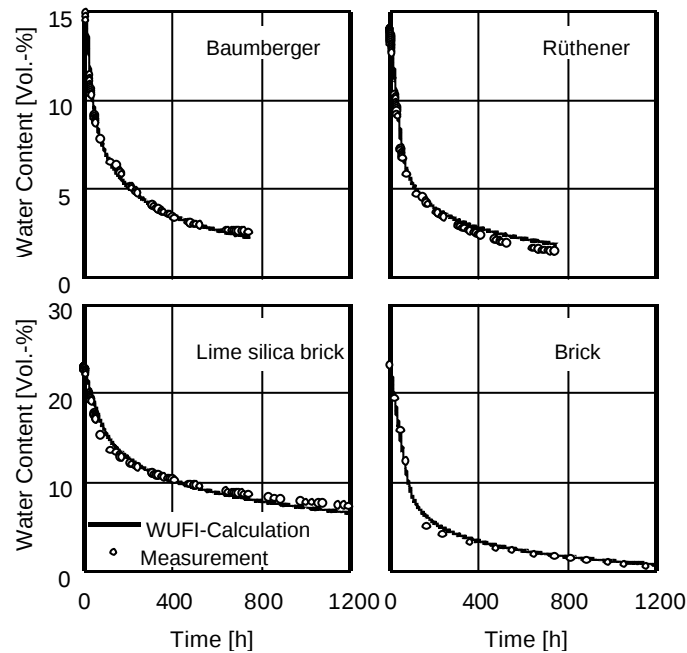
Fig. 4 Course of drying of initially saturated samples with one-sided drying at 20°C and 65% RH. The measured results are presented as dots, the calculated ones as a solid line.
