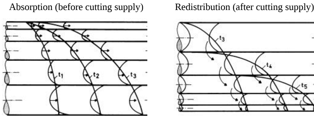
Fig. 1: Capillary transport phenomena represented by a model of interconnected cylindrical capillaries of various diameters.
