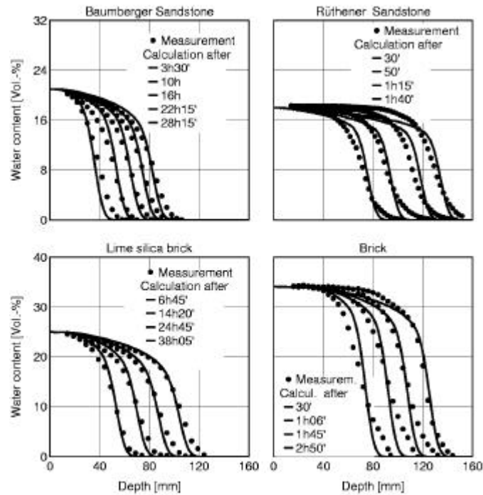
Fig. 3 Water content distributions over the depth of various building material samples at various times on the basis of NMR measurements and calculations of the absorption process.
