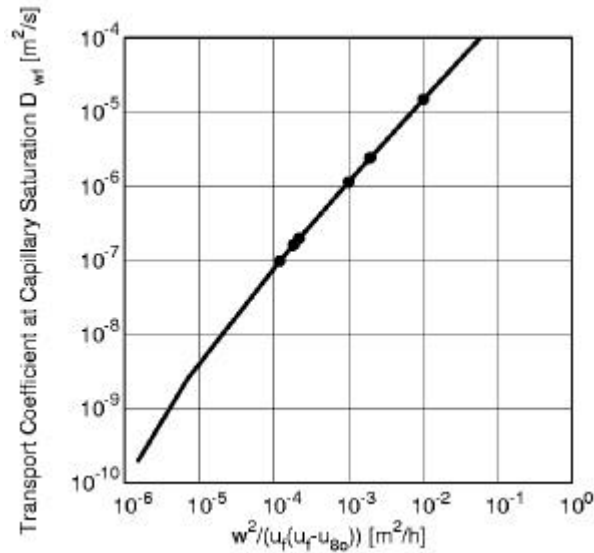
Fig. 2 Representation of Equation (3) for the graphical determination of D_w . The values for the materials listed are marked as dots.
